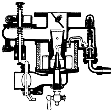
STROMBERG CARBURETOR—TYPE "B."
