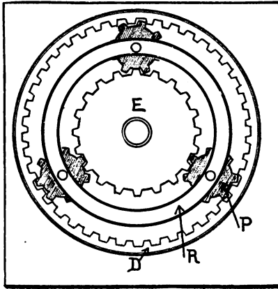
PRINCIPLE OF THE PLANETARY TRANSMISSION.
