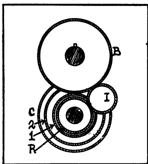
SELECTIVE SLIDING GEAR TRANSMISSION. (End Elevation.)
