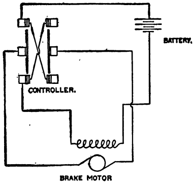
WIRING DIAGRAM OF HARTFORD ELECTRIC BRAKE.
