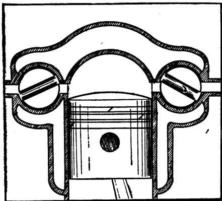
ROTARY VALVE ENGINE.
