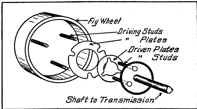
MULTIPLE DISC CLUTCH PARTS.
