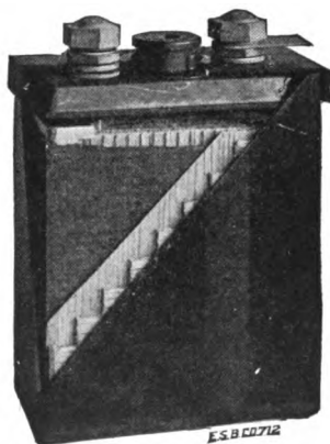
SECTION THROUGH LEAD STORAGE BATTERY CELL SHOWING ARRANGEMENT OF PLATES AND SEPARATORS.
