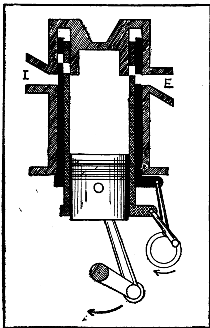
SLEEVE VALVE ENGINE.
