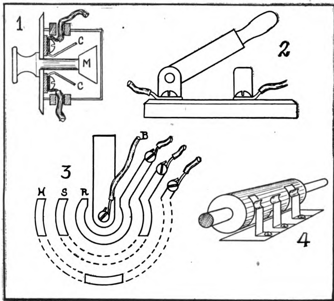
SWITCHES.
