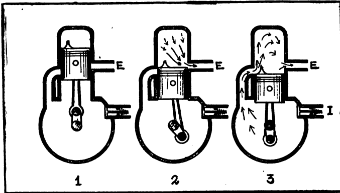
TWO PORT, TWO CYCLE ENGINE.
