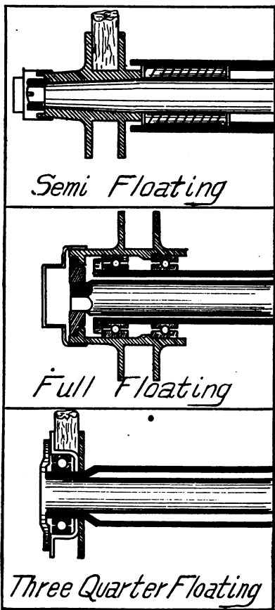
THREE TYPES OF LIVE REAR AXLES.
