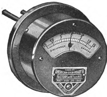
AMMETER FOR USE IN LIGHTING AND CHARGING CIRCUIT. Showing adjustment at lower part of front cover.
