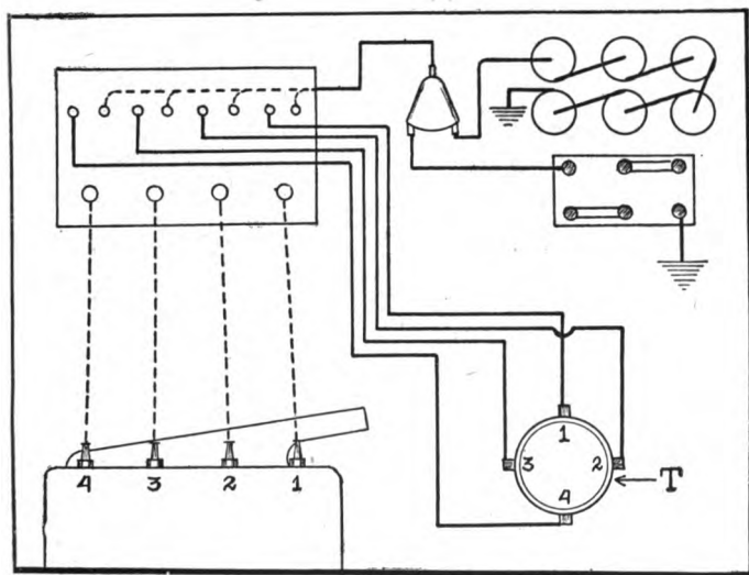
FOUR UNIT COIL AND TIMER WIRING.
