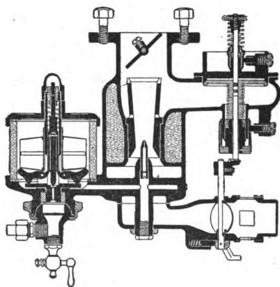
STROMBERG CARBURETOR—TYPE "A."
