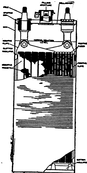
SECTION THROUGH EDISON BATTERY CELL.
