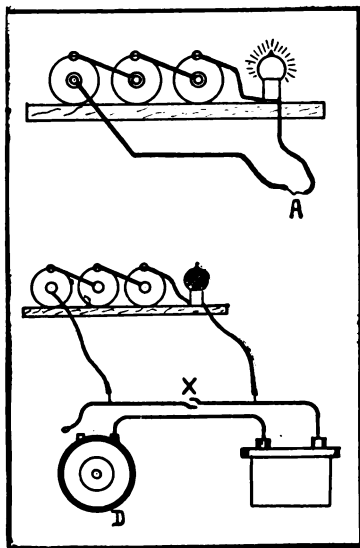
TESTER.
