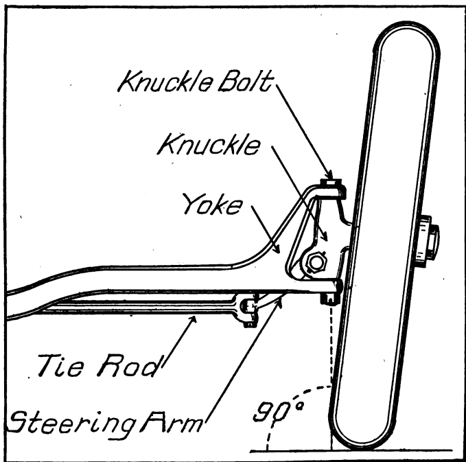
FRONT AXLE AND WHEEL.
