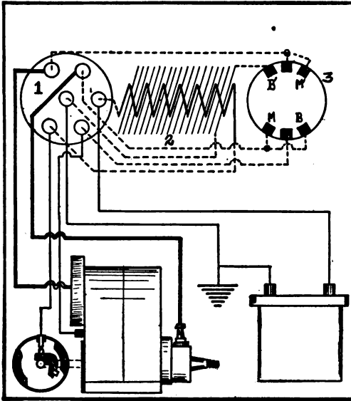
HIGH TENSION MAGNETO WITH SEPARATE BATTERY COIL.
