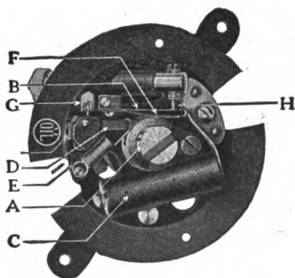
Fig. 11.—Contact maker disassembled.
