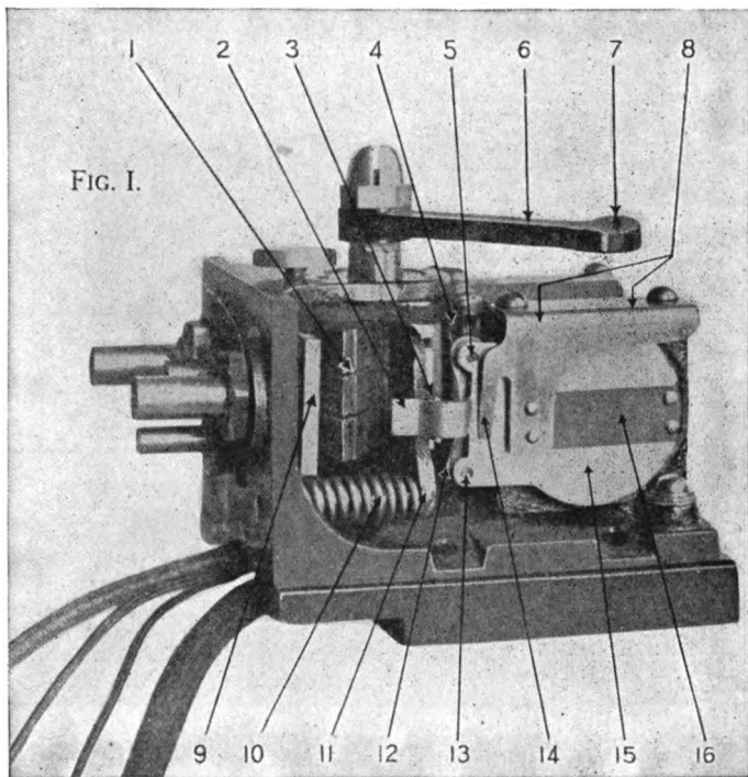
A MOTOR-GENERATOR CONTROLLER.
