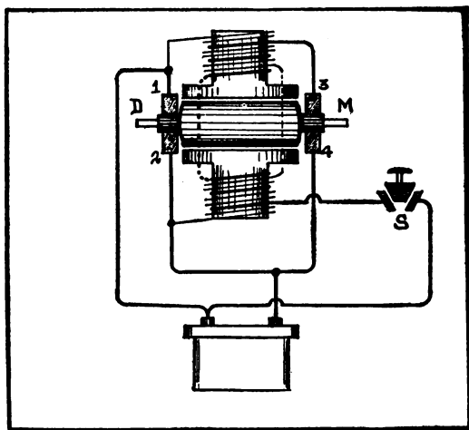
COMPOUND WOUND DYNAMO AND MOTOR.
