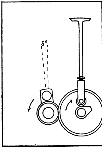
CAM AND VALVE OPENING MECHANISM.
