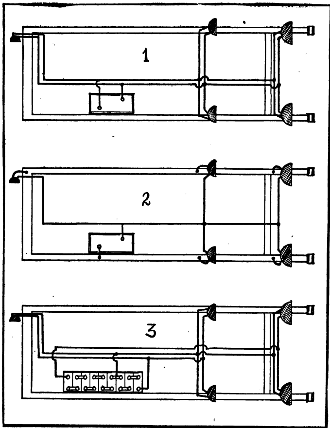
WIRING SYSTEMS.
