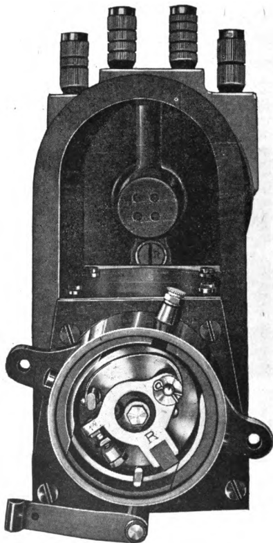
MAGNETO WITH BREAKER COVER REMOVED.
