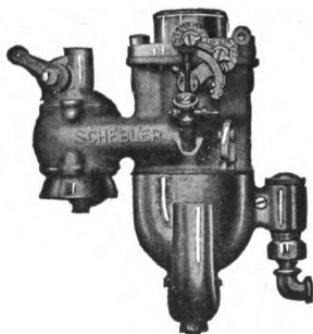
SCHEBLER MODEL L CARBURETOR.
