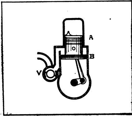
DIFFERENTIAL PISTON, TWO CYCLE ENGINE.
