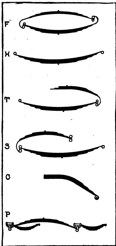
FORMS OF LEAF SPRINGS.
