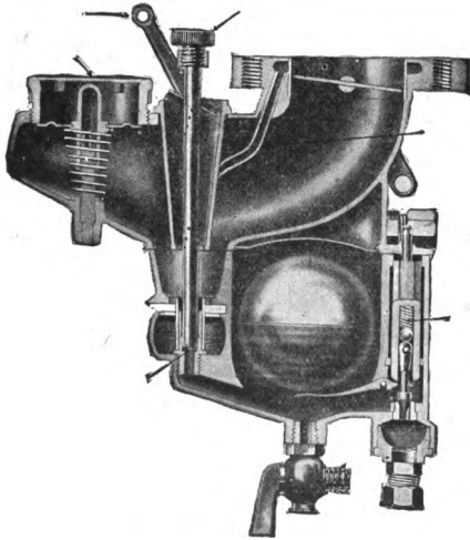
CARTER CARBURETOR.
