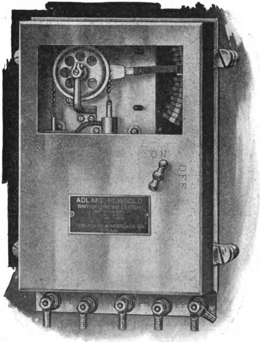
REGULATOR USING A SOLENOID WITH MOVABLE PLUNGER OPERATING A RHEOSTAT. CUT-OUT IS CONTAINED IN SAME CASE.
