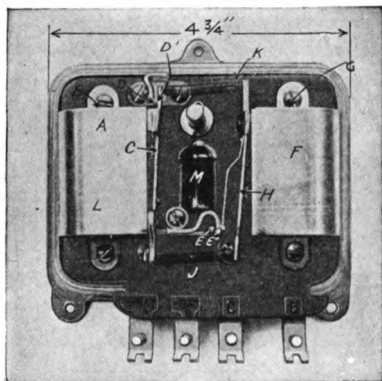
CONTROLLER AND CUT-OUT. (Ward Leonard.)
