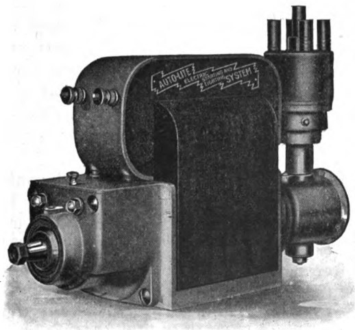
AUTOLITE DYNAMO, SHOWING HOW THE IGNITER IS ATTACHED.
