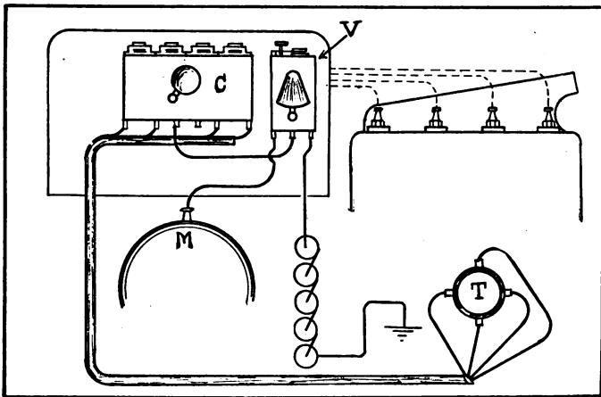
MASTER VIBRATOR WIRING.
