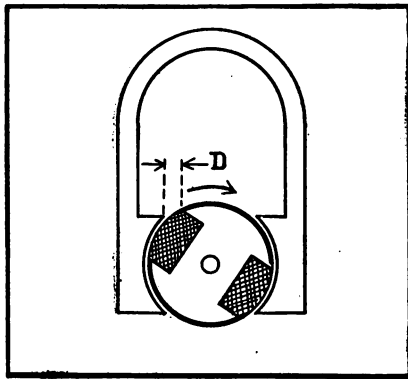
ARMATURE POSITION, D, Gap between edge of pole piece and edge of armature core.
