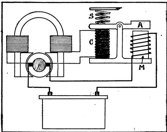
OUTPUT CONTROL, SHUNT FIELD RESISTANCE.
