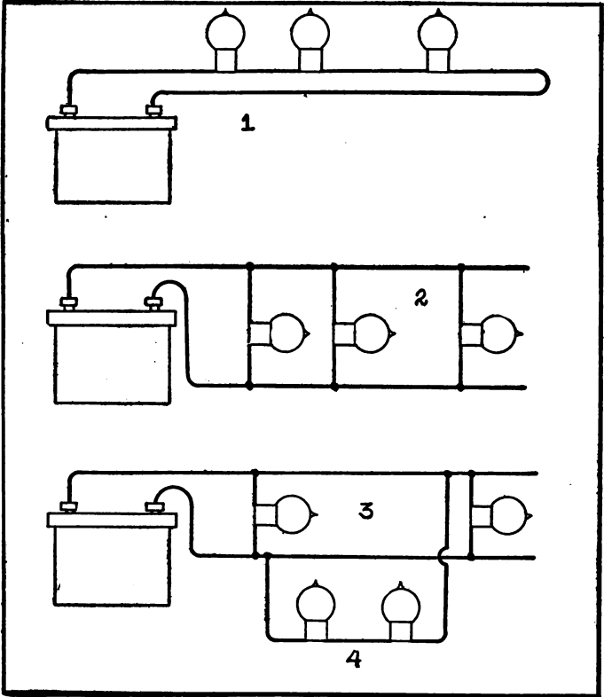
LAMP CONNECTIONS.
