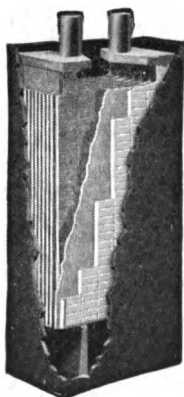
INTERIOR OF A STORAGE BATTERY.
