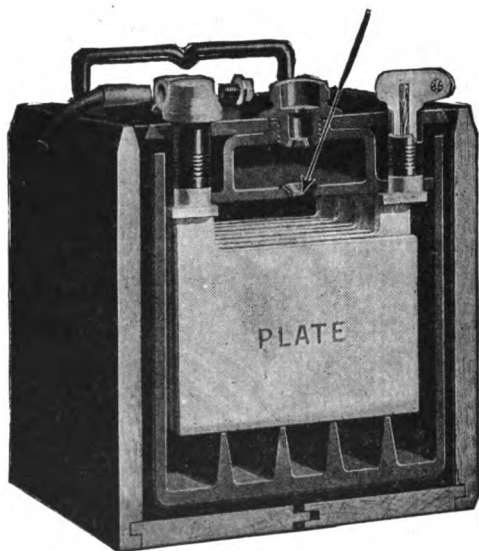
INTERIOR OF LEAD STORAGE BATTERY.
