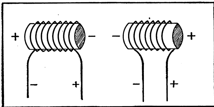
ELECTRO-MAGNETS.
