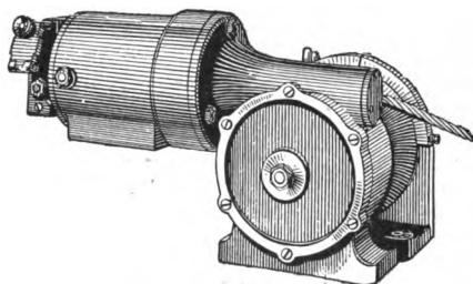
MOTOR AND CABLE DRUM OF ELECTRIC BRAKE.
