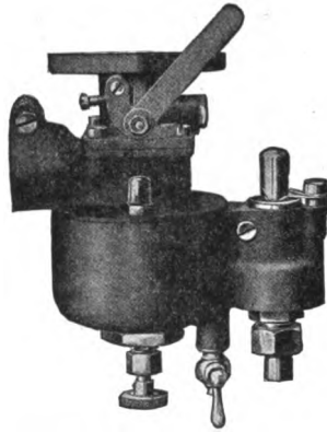
HOLLEY MODEL "H" CARBURETOR.
