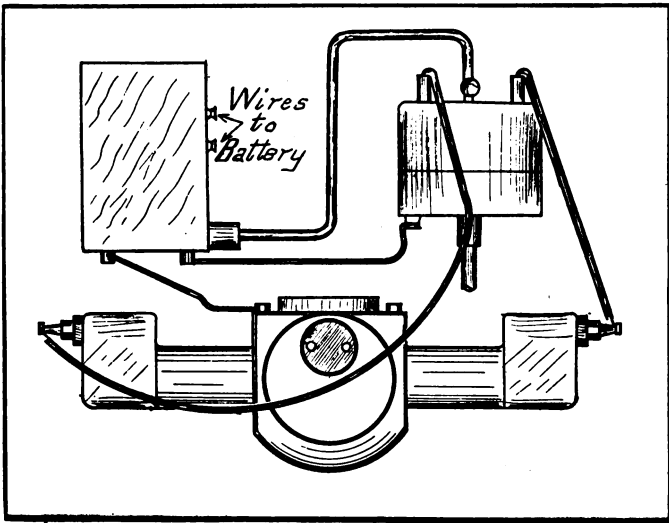
HIGH TENSION DISTRIBUTOR.
