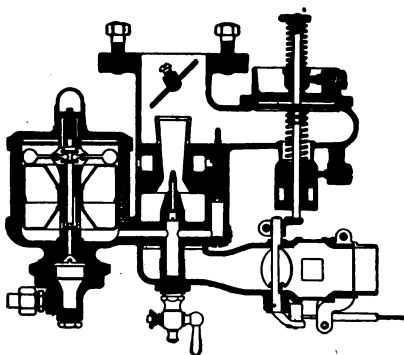
STROMBERG CARBURETOR—TYPE "G." Secondary gasoline jet in auxiliary air intake.
