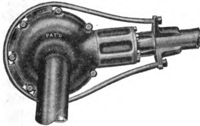
BRACE FOR STRENGTHENING REAR AXLE HOUSING.
