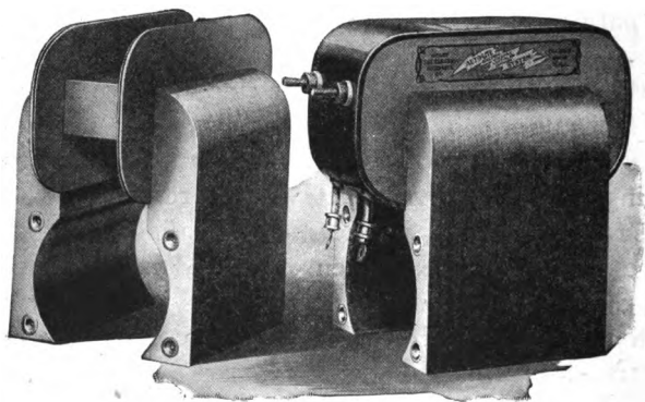
FIELD MAGNETS, BEFORE AND AFTER APPLYING THE WINDINGS.
