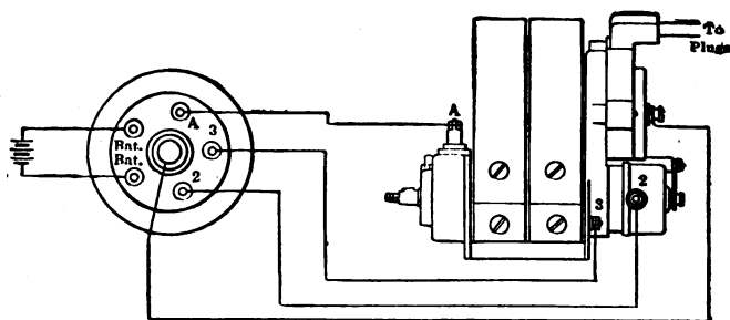
WIRING OF MAGNETO WITH DASH COIL. (Splitdorf.)
