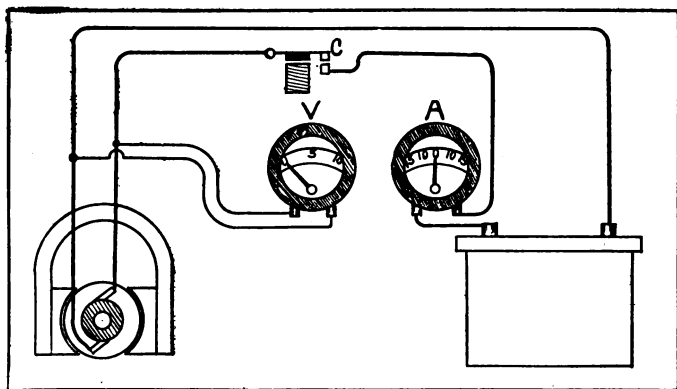
METER CONNECTIONS.
