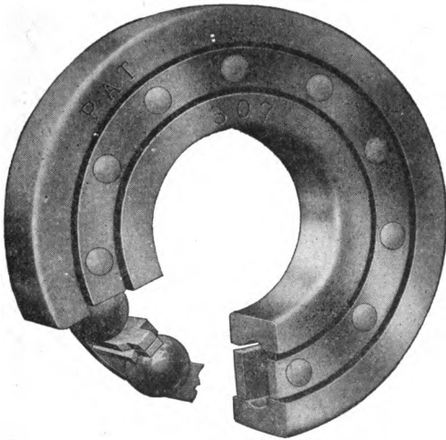
ANNULAR BALL BEARING.
