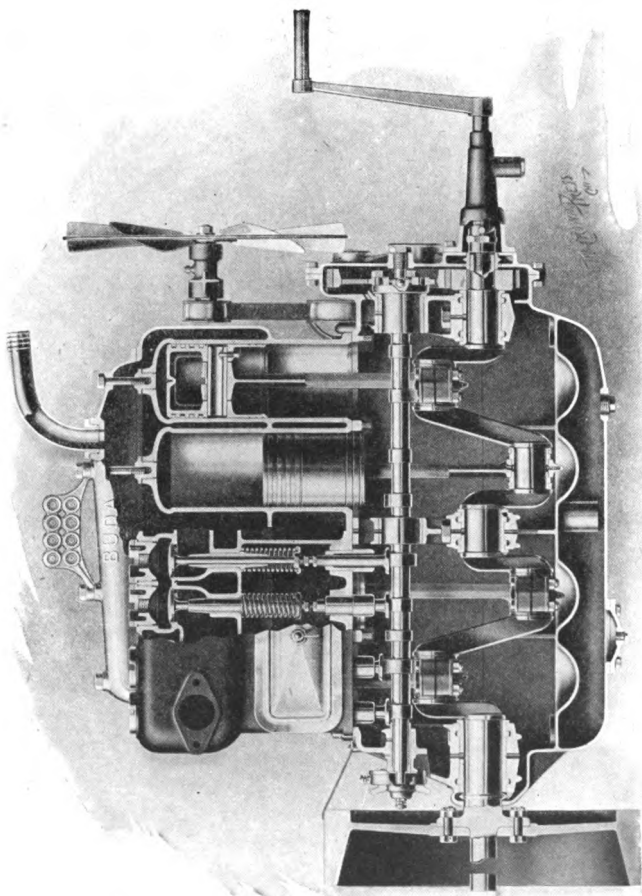
FOUR CYLINDER VERTICAL AUTOMOBILE ENGINE.
