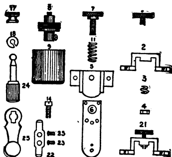
VIBRATOR AND COIL PARTS,
