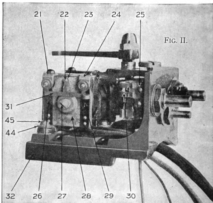
A MOTOR-GENERATOR CONTROLLER.
