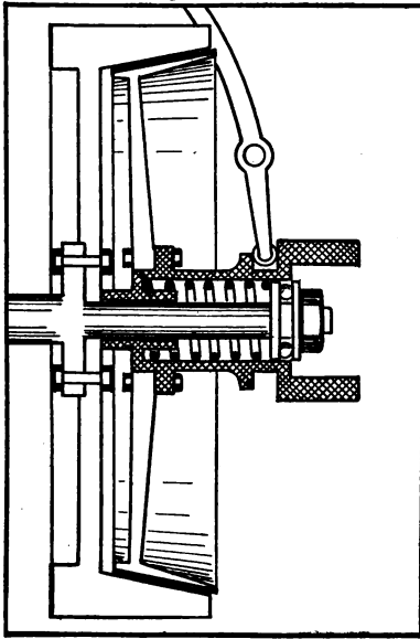
CONE CLUTCH.
