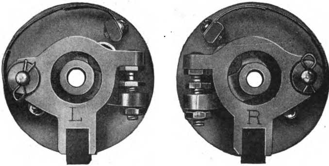
MAGNETO BREAKER.
