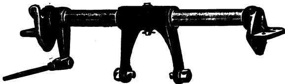
CROSS SHAFT AND ARMS FOR RELEASING CLUTCH.
