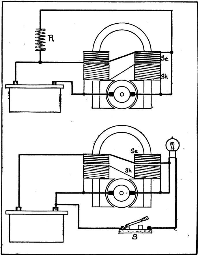
1 OUTPUT CONTROL, BUCKING COILS. Upper—Bosch-Rushmore system: R, Ballast coil; Sh, Shunt winding; Se, Series bucking coil. Lower—Bucking coil controlled through lamp circuit; S, light switch; Sh, Shunt field; Se, Bucking coil field.
