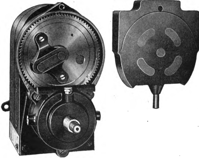
MAGNETO WITH DISTRIBUTOR COVER REMOVED.
