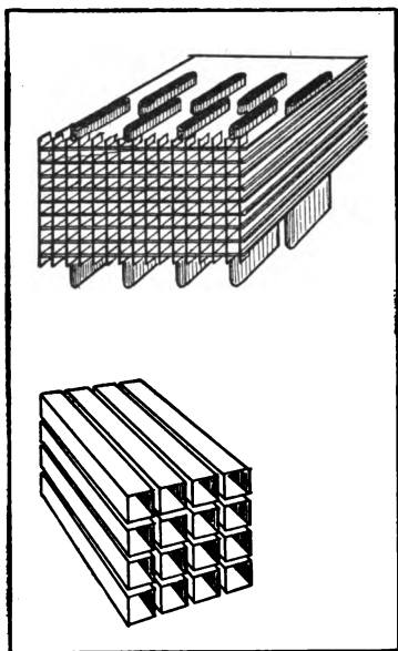
UPPER ILLUSTRATION—TUBULAR RADIATOR; LOWER ILLUSTRATION—CELLULAR RADIATOR.
