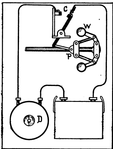
CENTRIFUGAL GOVERNOR CUT-OUT.
