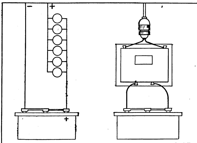
BATTERY CHARGING. Through lamp resistance or through rectifier.
