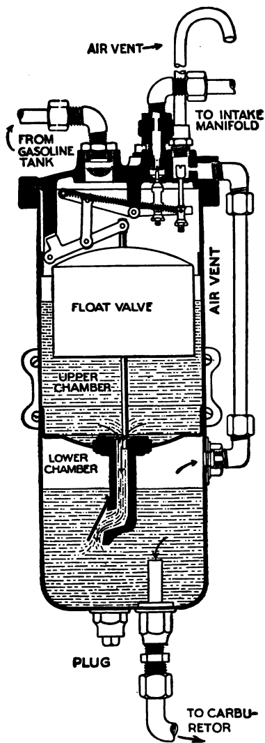
VACUUM FUEL FEED SYSTEM. (Stewart-Warner.)
