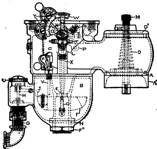
SCHEBLER MODEL L CARBURETOR.
