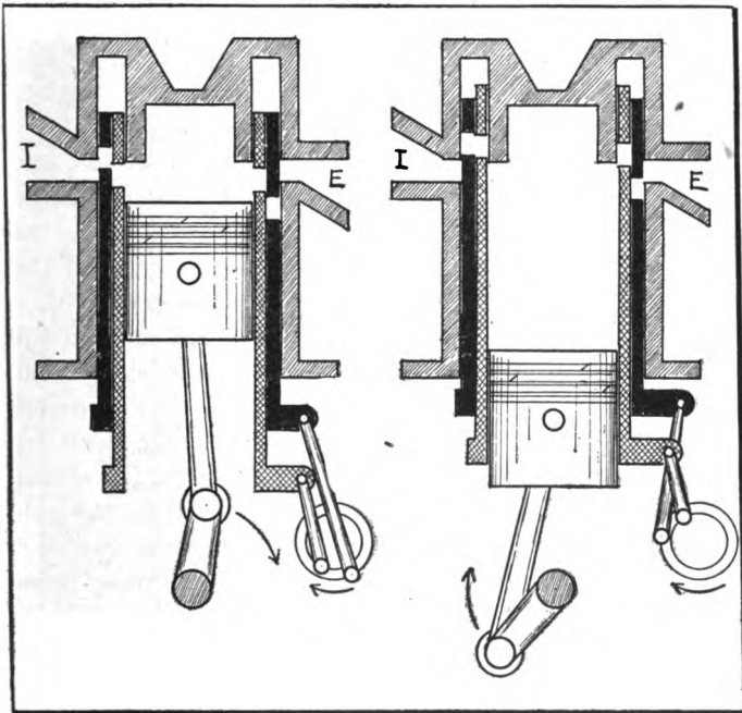
SLEEVE VALVE ENGINE.
