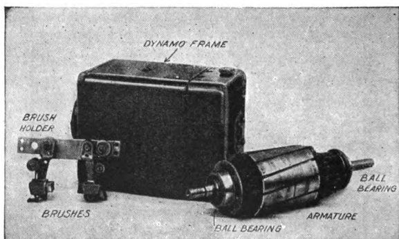
DYNAMO PARTS.
