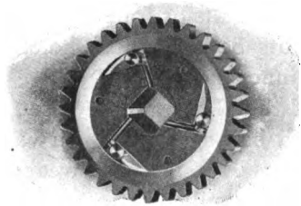
OVERRUNNING CLUTCH, ROLLER TYPE.
