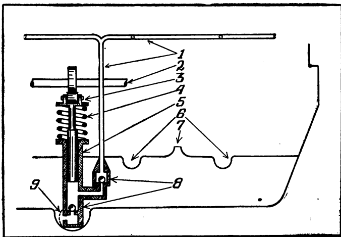
CIRCULATING OILING SYSTEM IN ENGINE CRANK CASE.
