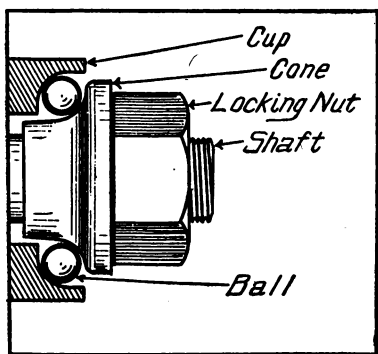
CUP AND CONE BALL BEARING APPLICATION.
