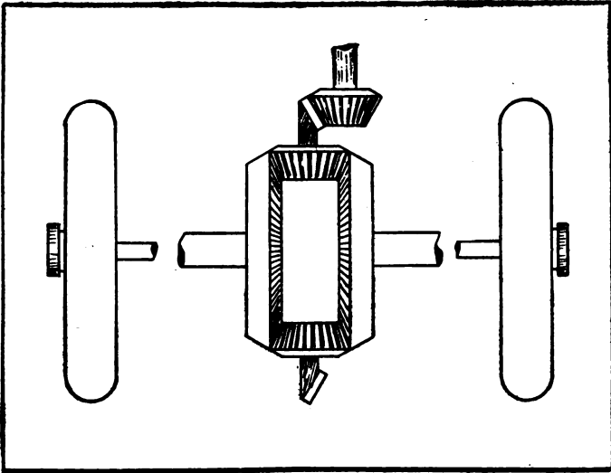
PRINCIPLE OF THE DIFFERENTIAL.
