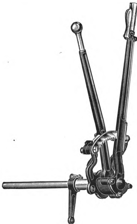
EMERGENCY BRAKE HAND LEVER AND GEAR SHIFT HAND LEVER.
