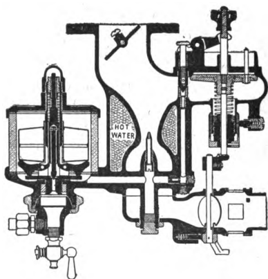
STROMBERG CARBURETOR—TYPE "C." Showing secondary gasoline jet operated by air valve.
