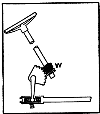
WORM AND SECTOR STEERING GEAR.
