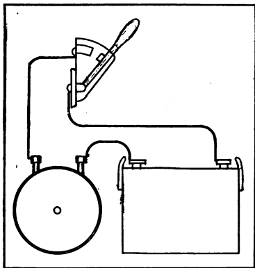
HAND OPERATED CUT-OUT.
