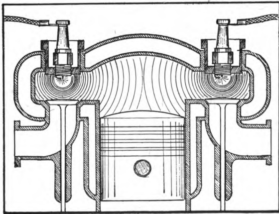
EFFECT OF TWO SPARK IGNITION.
