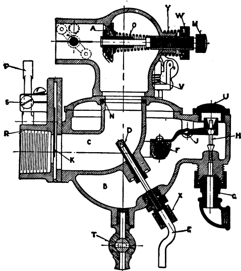
SCHEBLER MODEL D CARBURETOR.
