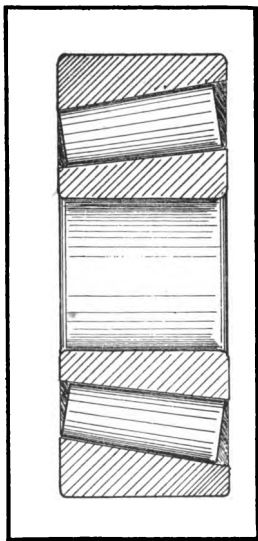
ROLLER BEARING.
