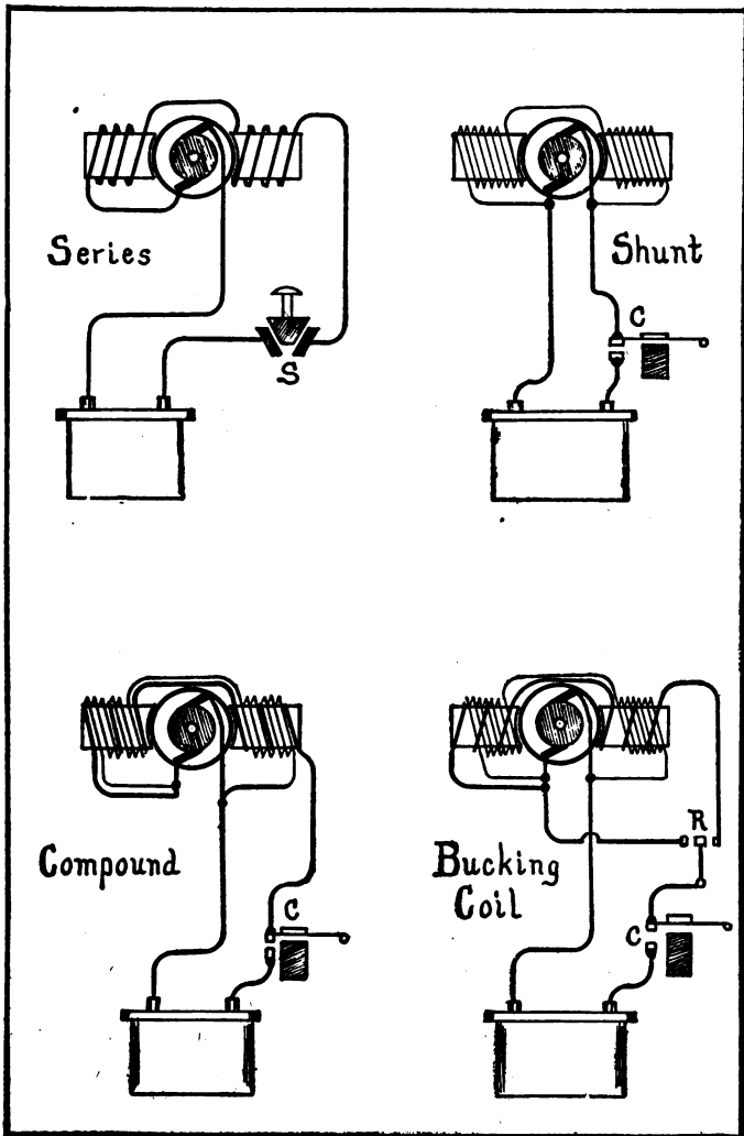
FIELD WINDINGS.
