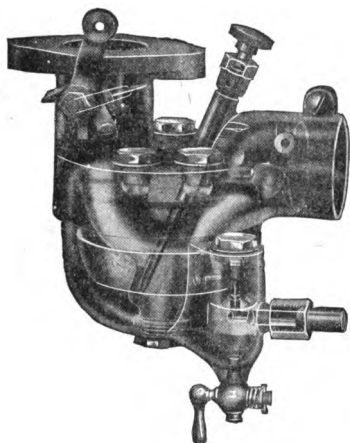
KINGSTON CARBURETOR.
