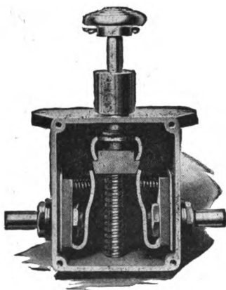
TYPICAL STARTING SWITCH.
