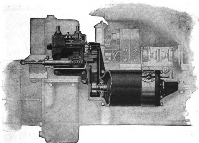
STARTING MOTOR INSTALLATION.
