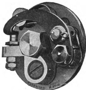
MAGNETTO BREAKER. (Splitdorf.)
