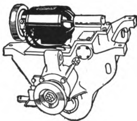
STARTING MOTOR DRIVING INTO TRANSMISSION GEARS.
