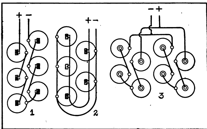
DRY CELL CONNECTIONS. 1, Series; 2, Multiple; 3, Multiple-Series.
