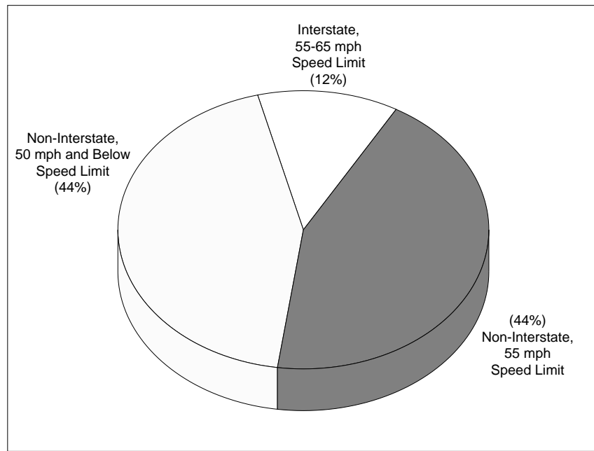
Figure 7. Speed-Related Fatalities by Road Type, 1994
