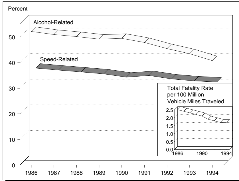
Figure 5. Percentages of Fatalities Related to Speed and to Alcohol, 1986-1994
