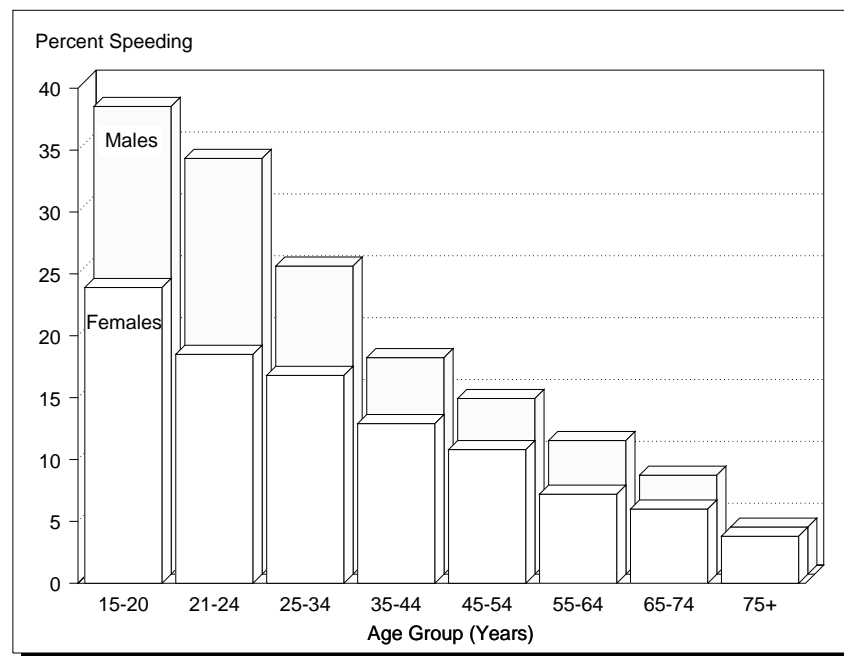
Figure 2. Speeding Drivers in Fatal Crashes by Age and Sex, 1994
