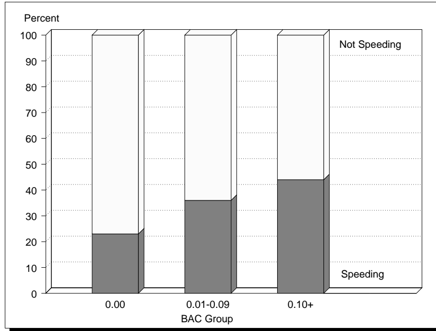
Figure 3. All Drivers Involved in Fatal Crashes by BAC Level and Speed Status, 1994
