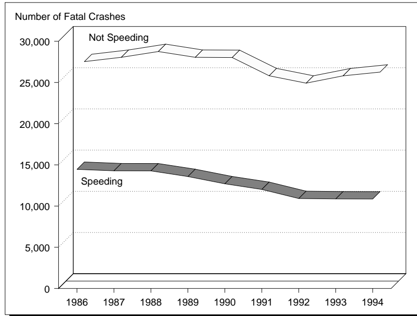
Figure 1. Fatal Crashes by Speed Status, 1986-1994
