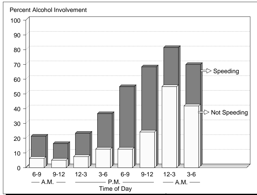
Figure 4. Drivers in Fatal Crashes by Alcohol Involvement, Speed Status, and Time of Day, 1994
