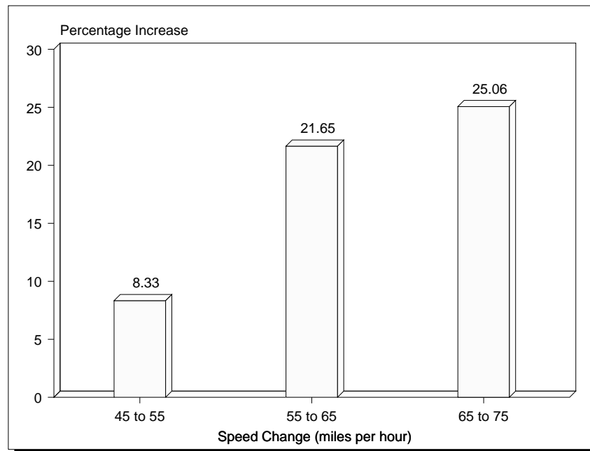
Figure 8. Percentage Increases in Fuel Consumption with Increasing Speeds
