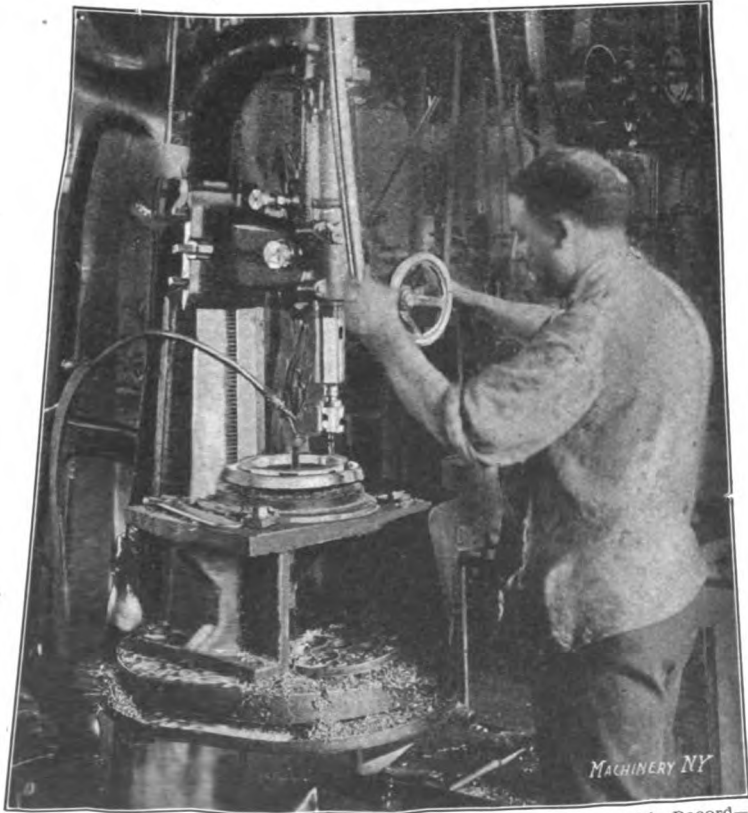
Fig. 45. A Tapping Operation and Operator with a Remarkable Record—75,000 Blind 5-16-inch Holes in Chrome-nickel Steel without breaking a Tap
