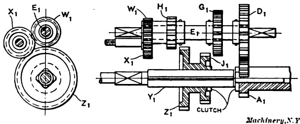
Fig. 8. Sketch showing Arrangement of Gears in Transmission Case
