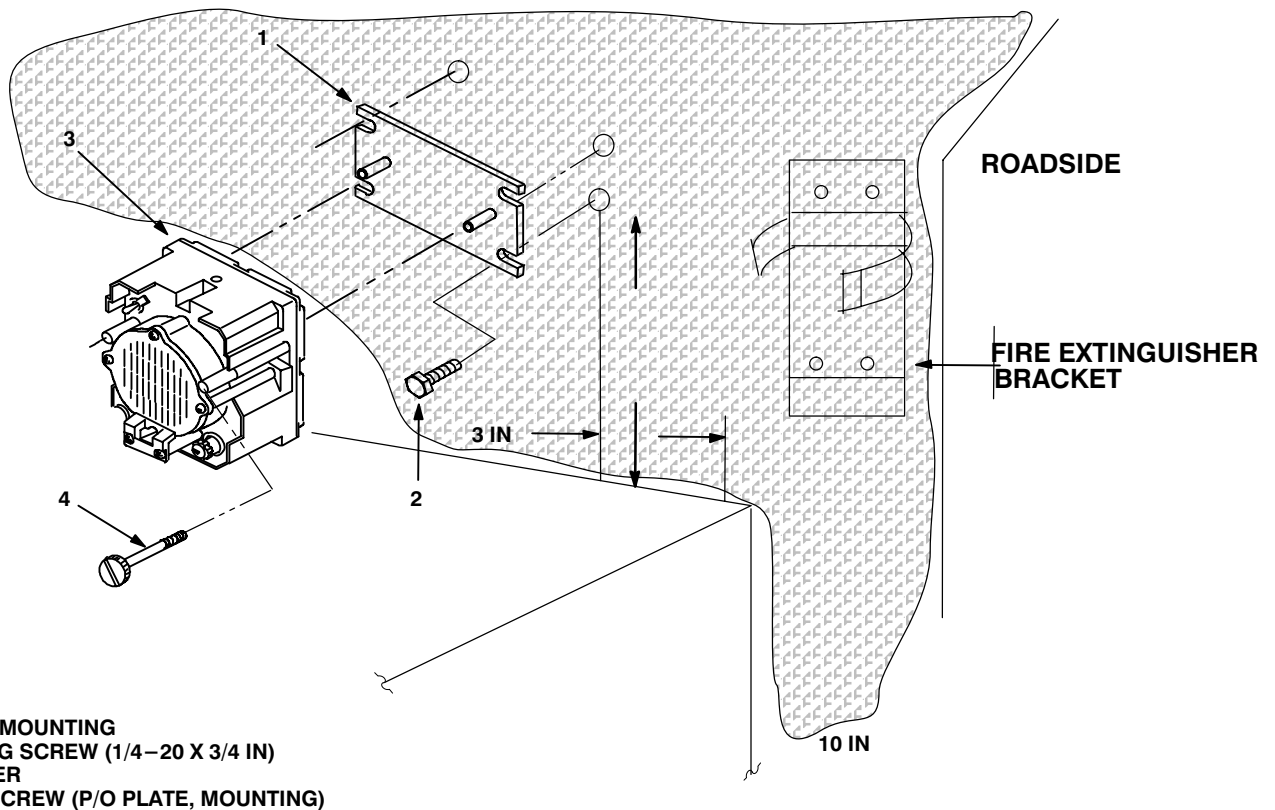
Figure 5-7. Speaker Installation
