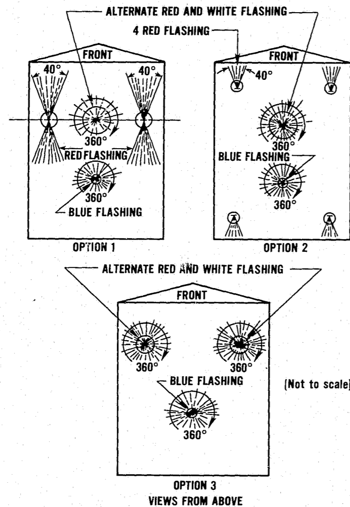
FIGURE 2. Rooftop installation configurations for emergency vehicle warning lights. Option 2 is recommended for fire engines and other long emergency vehicles to mark the rear corners of such vehicles. Options 1 and 3 are alternate, but less preferred configurations for long vehicles. Options 1, 2, and 3 are all equally acceptable for sedan-based vehicles. Blue flashing lights are for use on emergency vehicles during non-emergency situations.
