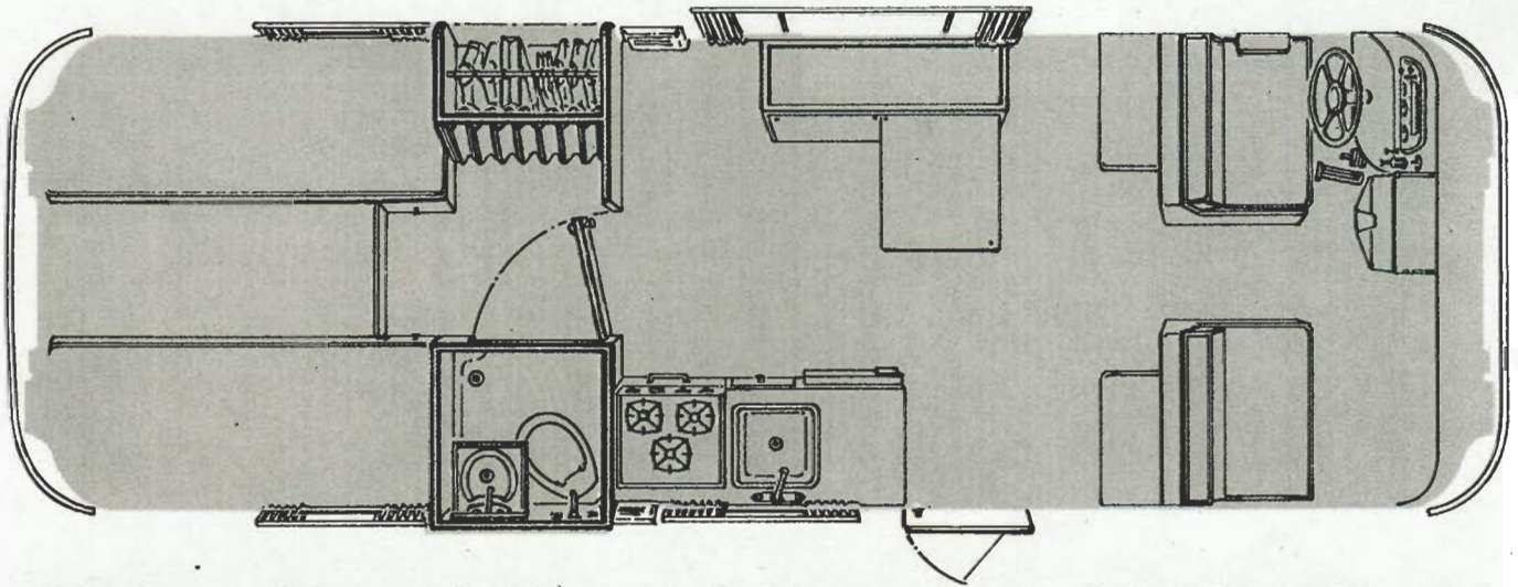
FLOOR PLAN FOR MODELS 400 AND 500
