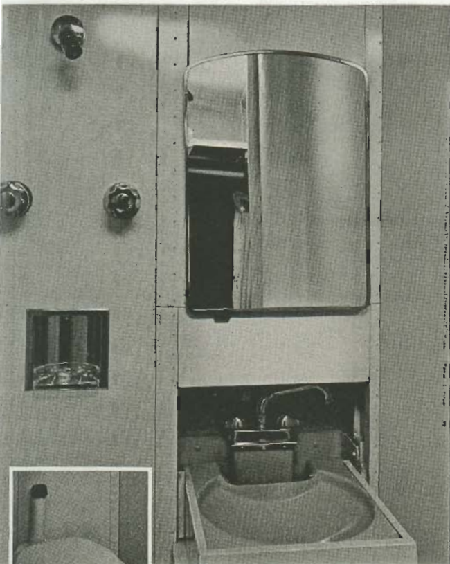
Complete bath facilities include shower, Pullman concealed wash basin and marine toilet. A 45-gallon storage tank with an automatic water pump and a 40-gallon holding tank with sewer connection maintain adequate plumbing for the unit.
